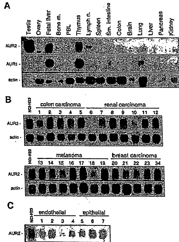
Fig. 4. Expression of human aurora1 and aurora2 . (A) Northern blot containing poly(A) + mRNA (2 \mu g per lane) from normal human tissue hybridized with an aurora1 or aurora2 DNA probe. (B) Aurora2 Northern blots containing total RNA (20 \mu g) from human tumor cell lines. The single 2.4 kb aurora2 transcript is marked. RNA from the lung cancer cell line NCI-H23 was included as a standard for the tumor blots. Cell lines included are: 1, HT-29; 2, HCC-2998; 3, COLO 205; 4, HCT-15; 5, KM012; 6, UO-31; 7, SN12C; 8, CAKI-1; 9, RFXP393; 10, ACHN; 11, 786-0; 12, TK-10; 13, LOX IMVI; 14, SK-MEL-2; 15, SK-MEL-5; 16, SK-MEL-28; 17, UACC-62; 18, UACC-257; 19, M14; 20, MCF-7/ADR-RES; 21, HS 578T; 22, MDA-MB-435; 23, MDA-N; 24, T-47D. (C) Aurora2 Northern blot containing total RNA (10 \mu g) from cultured primary human endothelial and epithelial cells. The single 2.4 kb aurora2 transcript is marked. RNA from the lung cancer cell line NCI-H23 was included as a standard for the blots. Primary cell RNAs are: 1, coronary artery endothelial cells; 2, pulmonary artery endothelial cells; 3, lung microvascular endothelial cells; 4, dermal microvascular endothelial cells; 5, mammary epithelial cells; 6, renal proximal tubule epithelial cells; and 7, renal cortex epithelial cells.
